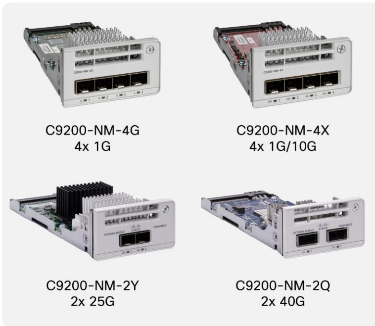
Figure 2. Cisco Catalyst 9200 Series Switch network modules
