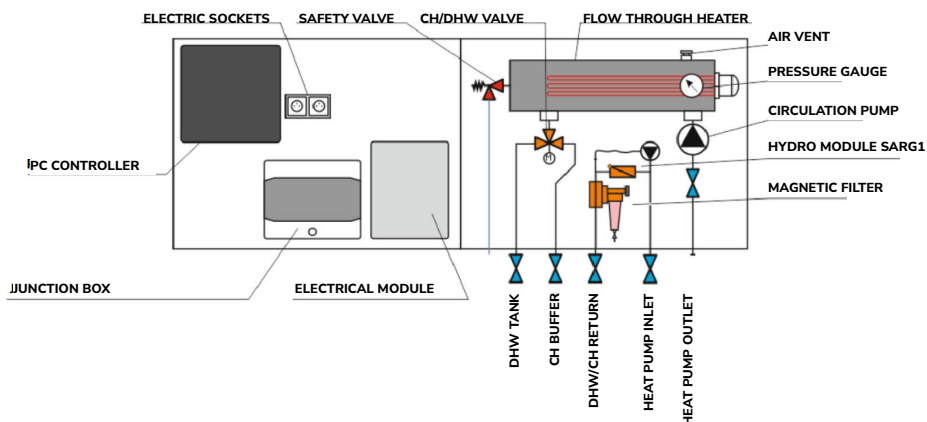
FIG. 2. COMPONENTS AND DESCRIPTION OF HYDRAULIC CONNECTIONS
