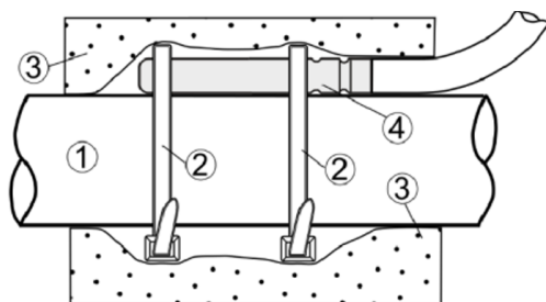
Installation of a circulating water temperature sensor: 1 - pipe, 2 - clamp, 3 - thermal insulation (insulation lagging), 4 - temperature sensor
