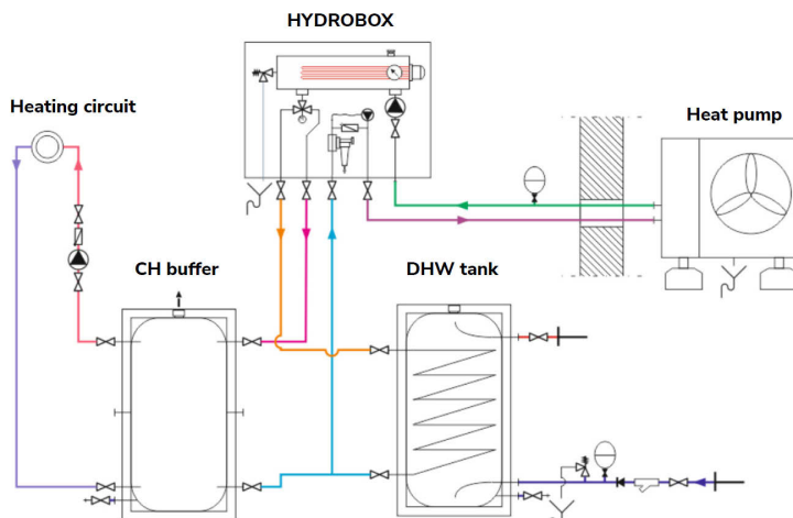
FIG. 1. EXAMPLE INSTALLATION DIAGRAM USING HYDROBOX MODULE KTH1
