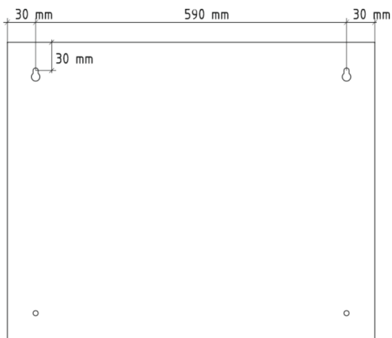
FIG. 4. INSTALLATION HOLES
