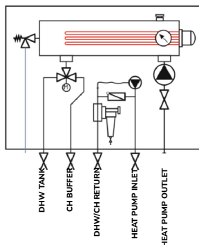
FIG. 5. HYDRAULIC CONNECTIONS
